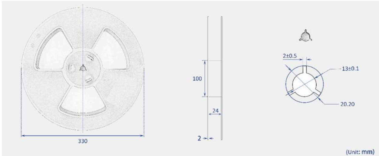
Figure 13 Reel dimensions
