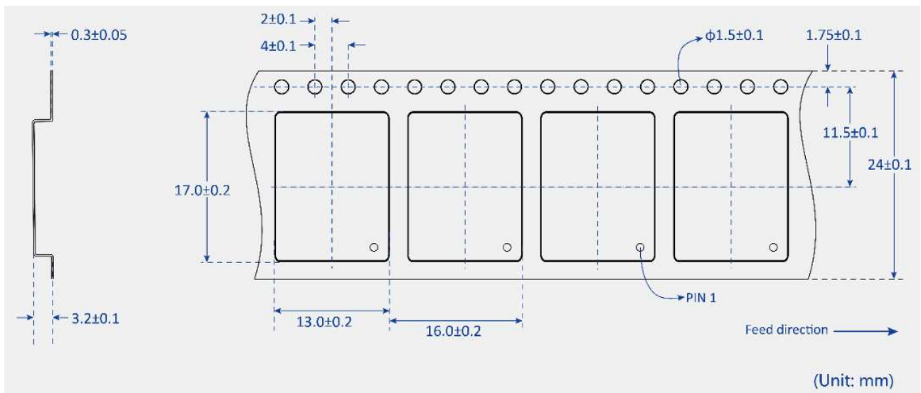
Figure 12 Tape dimensions
